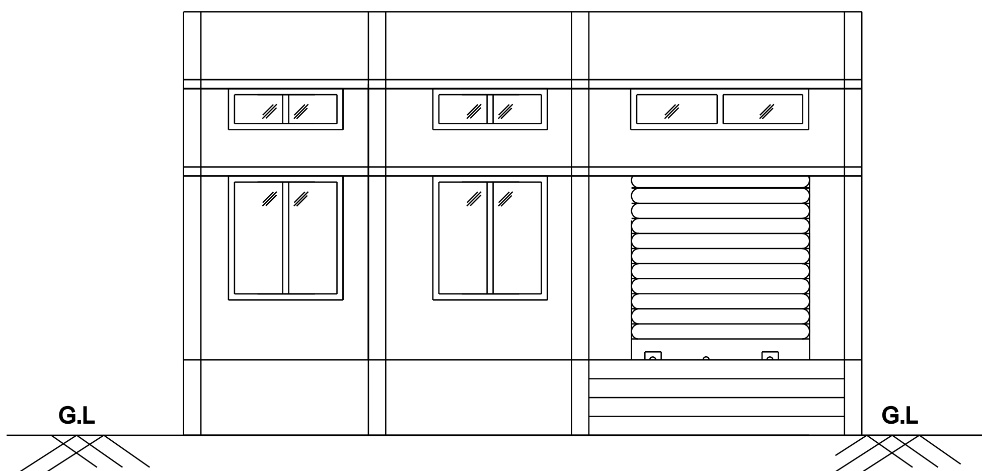
FRONT ELEVATION
