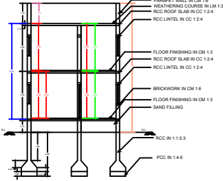
CROSS SECTION
