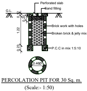
RAINWATER HARVESTING
