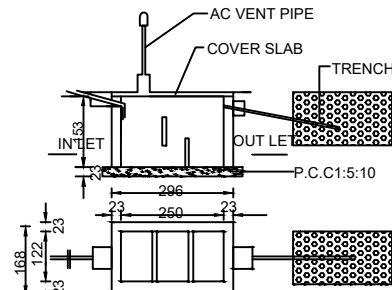
SEPTIC TANK
