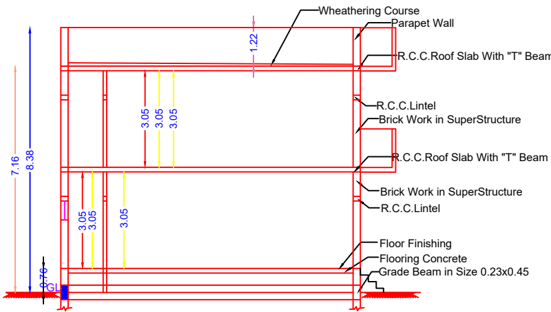
SECTION ON "PQ"
