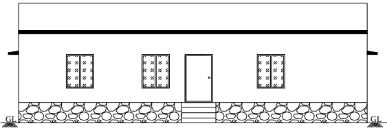
FRONT ELEVATION
