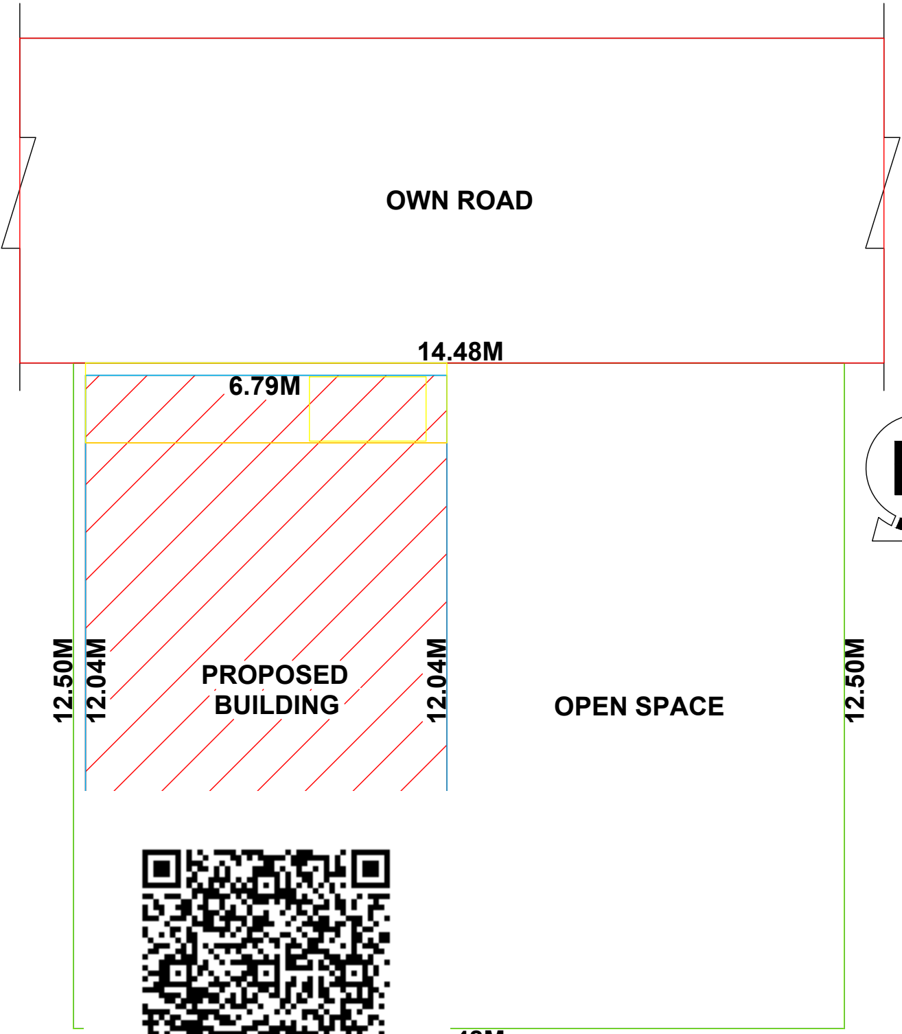
PLAN
