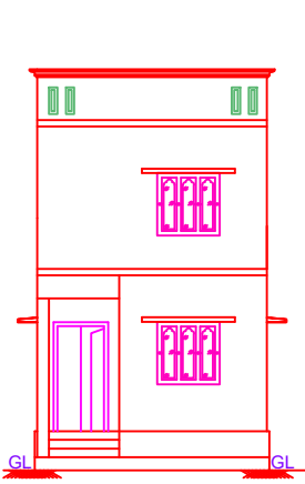
FRONT ELEVATION
