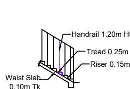
DETAILS OF STAIR CASE (SCALE 1:100)
