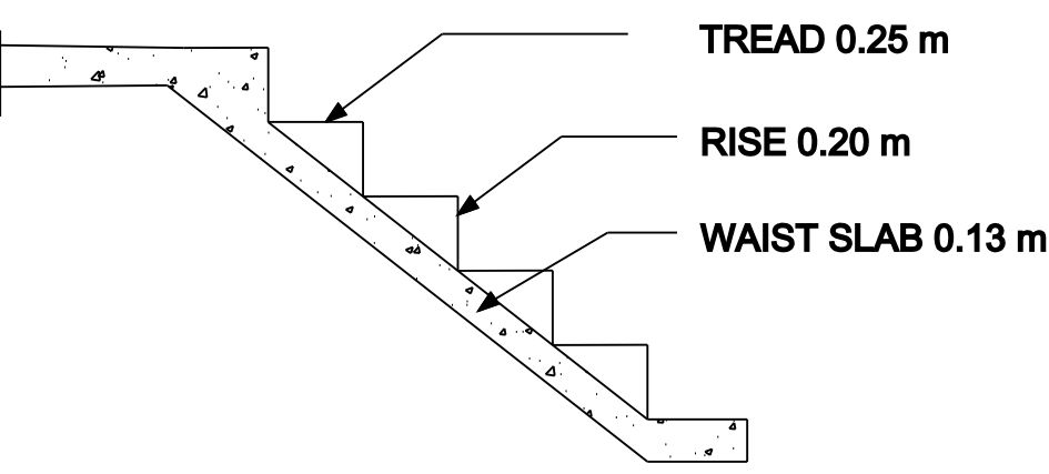
STAIR DETAILS
