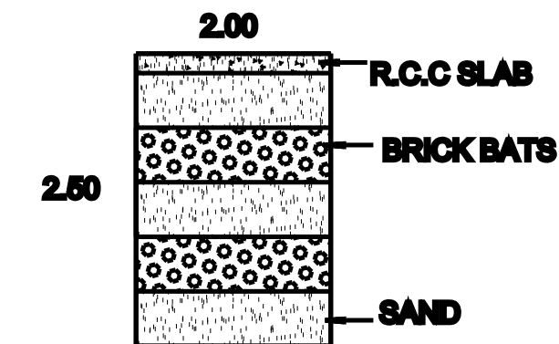
SECTION ON C - D
