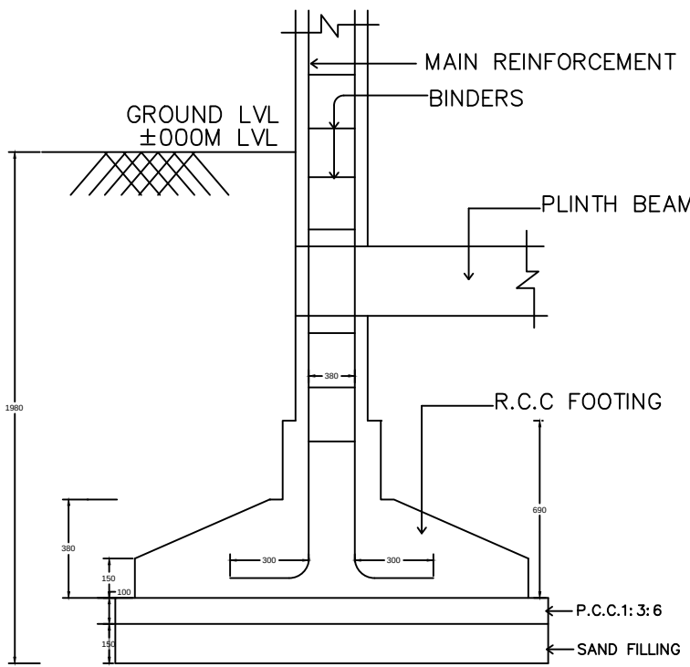
TYPICAL SECTION OF R.C.C COLUMN FOUNDATION
