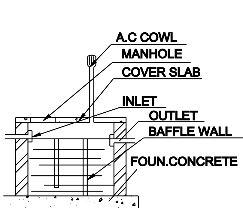
DETAILS OF SEPTIC TANK
