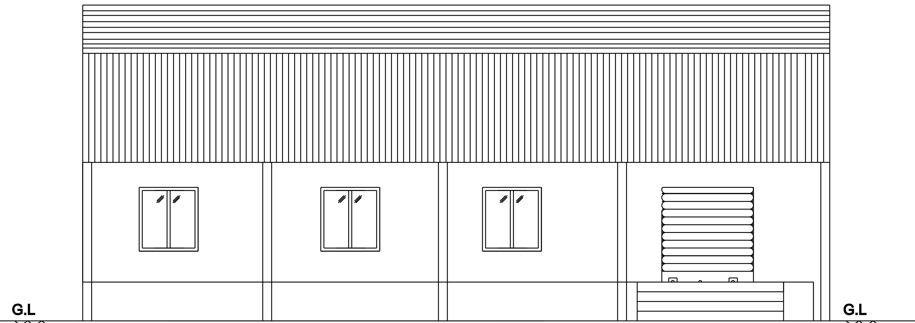
FRONT ELEVATION
