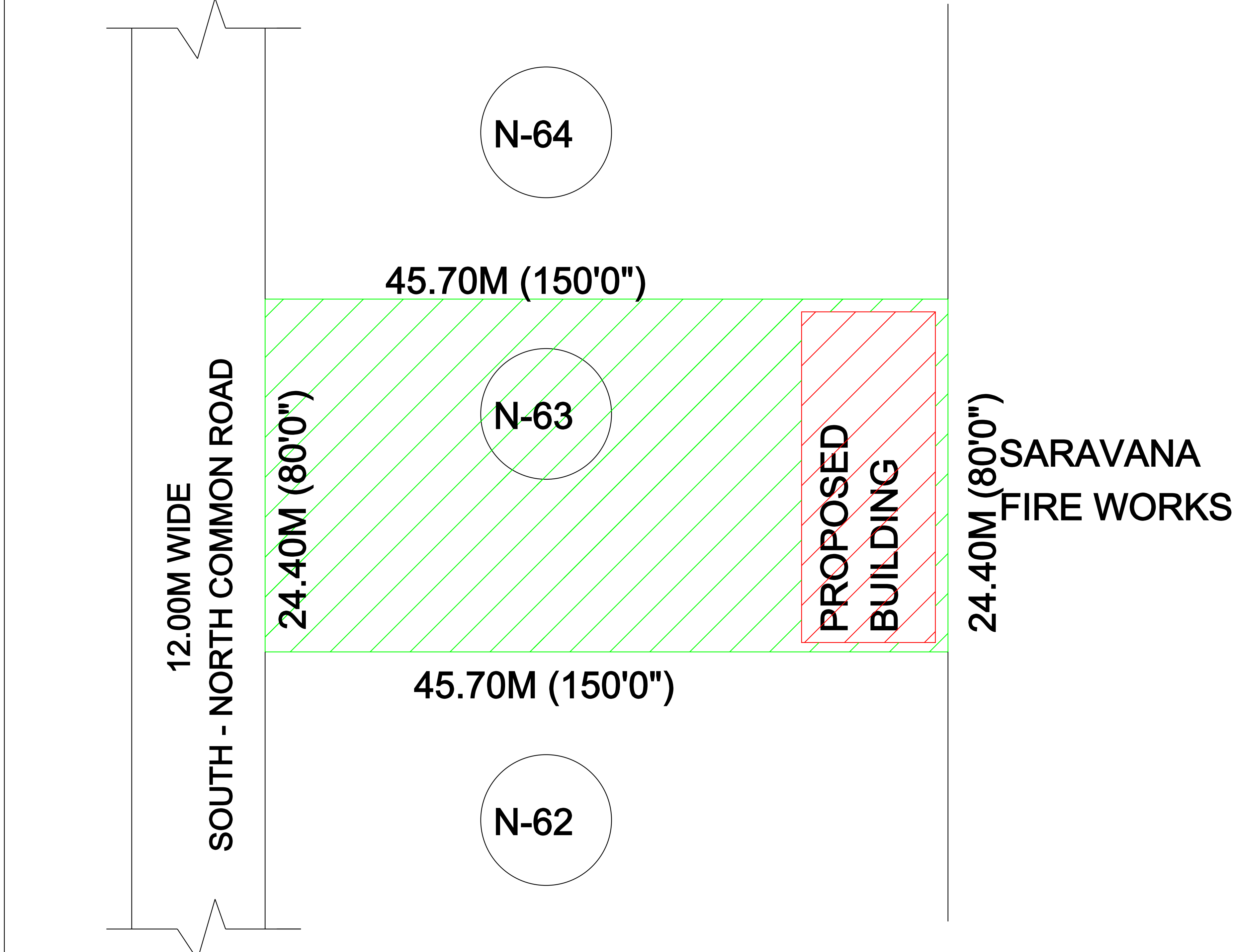
LOCATION PLAN
