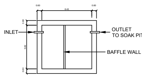
SEPTIC. TANK
