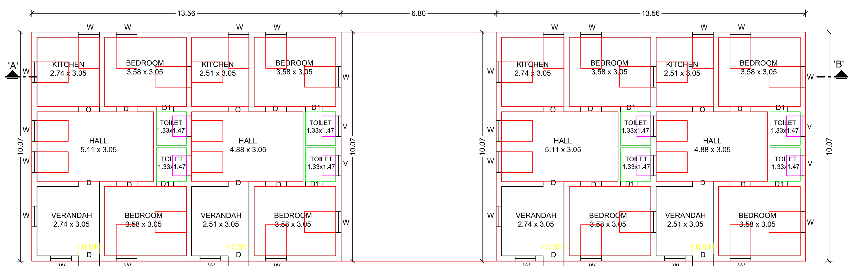
PLAN
