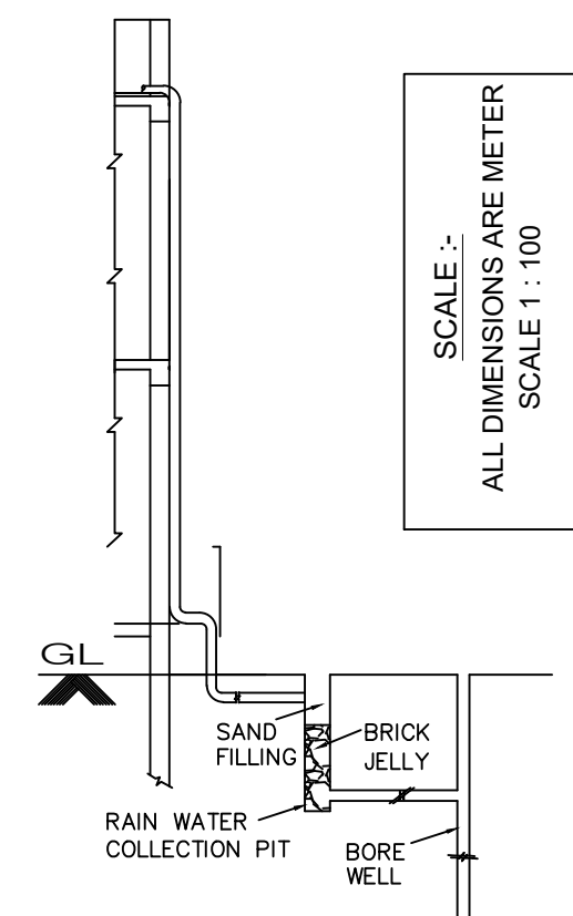
RAIN WATER HARVESTING SYSTEM
