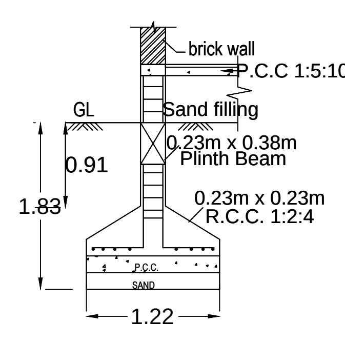
FOUNDATION DETAILS
