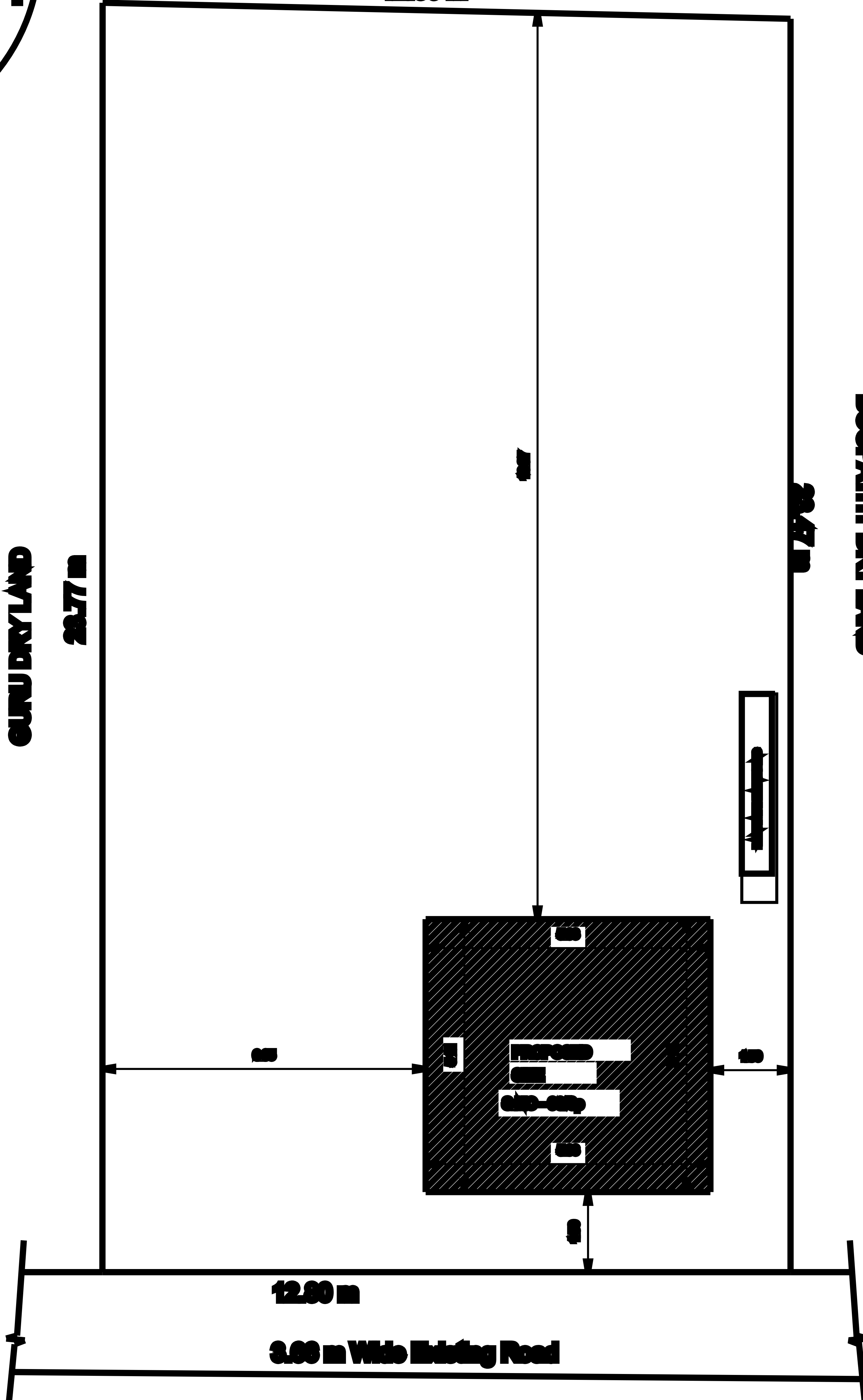
SITE PLAN
