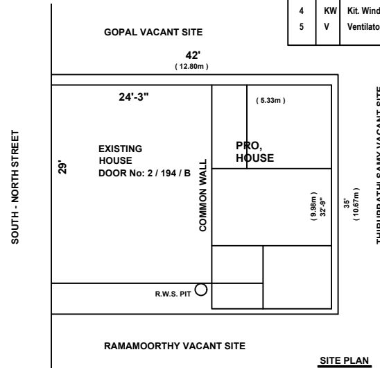
SITE PLAN
