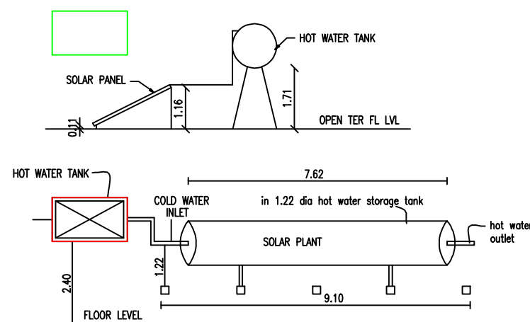
SOLAR WATER HEATER PLANT DETAILS
