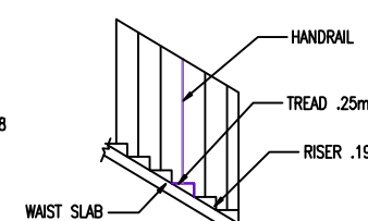
STAIR DETAIL
