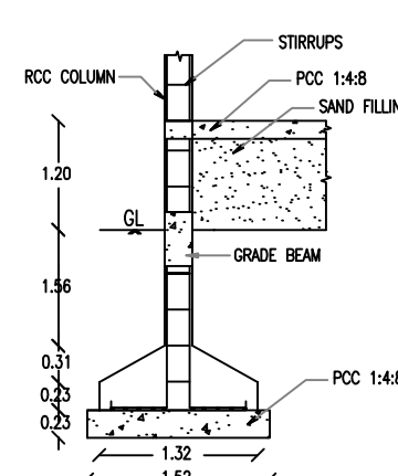
COLUMN DETAILS
