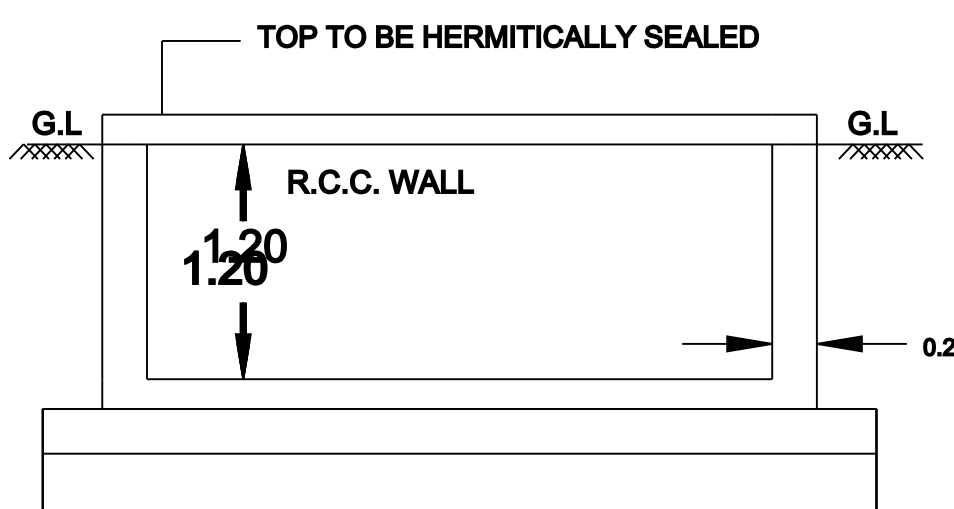
RWH_SECTION
