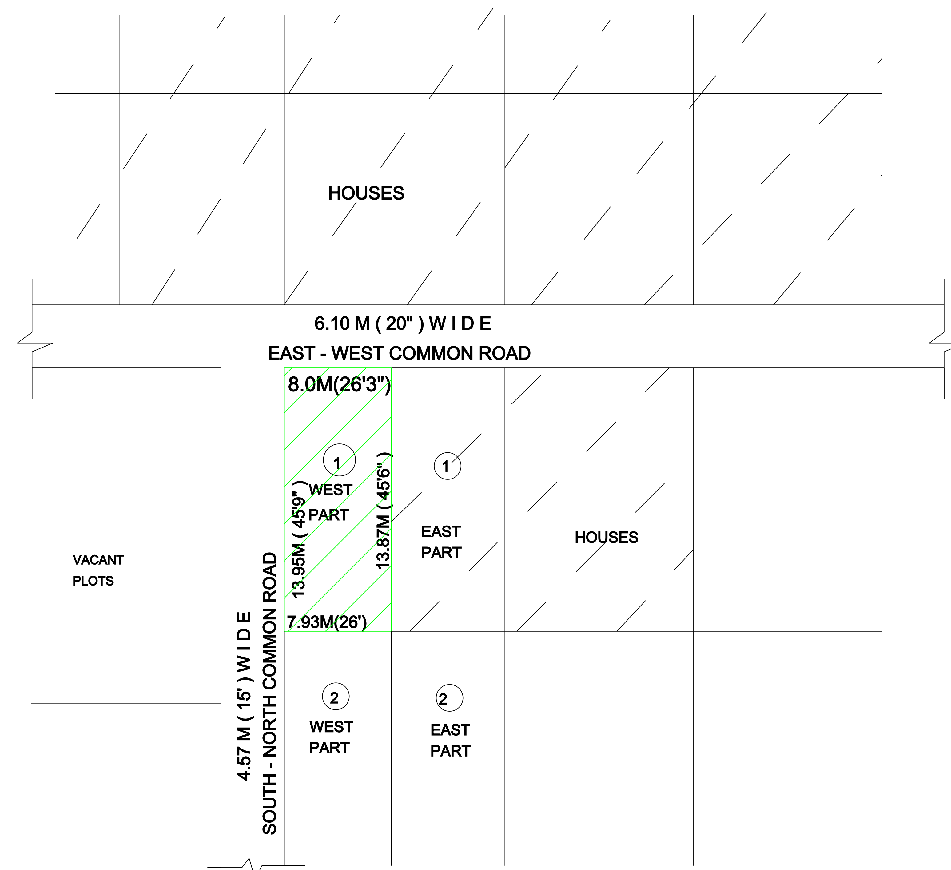
LOCATION PLAN
