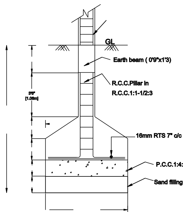
FOUNDATION DETAILS
