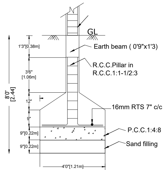
FOUNDATION DETAILS
