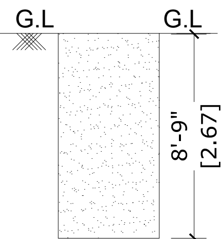
TRIAL PIT.
