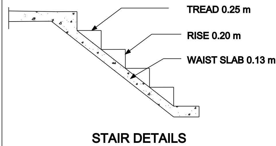
STAIR DETAILS
