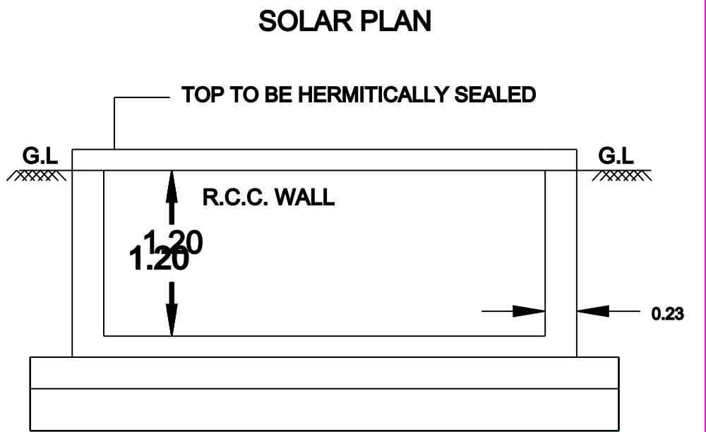
RWH SECTION
