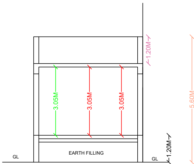
SECTION
