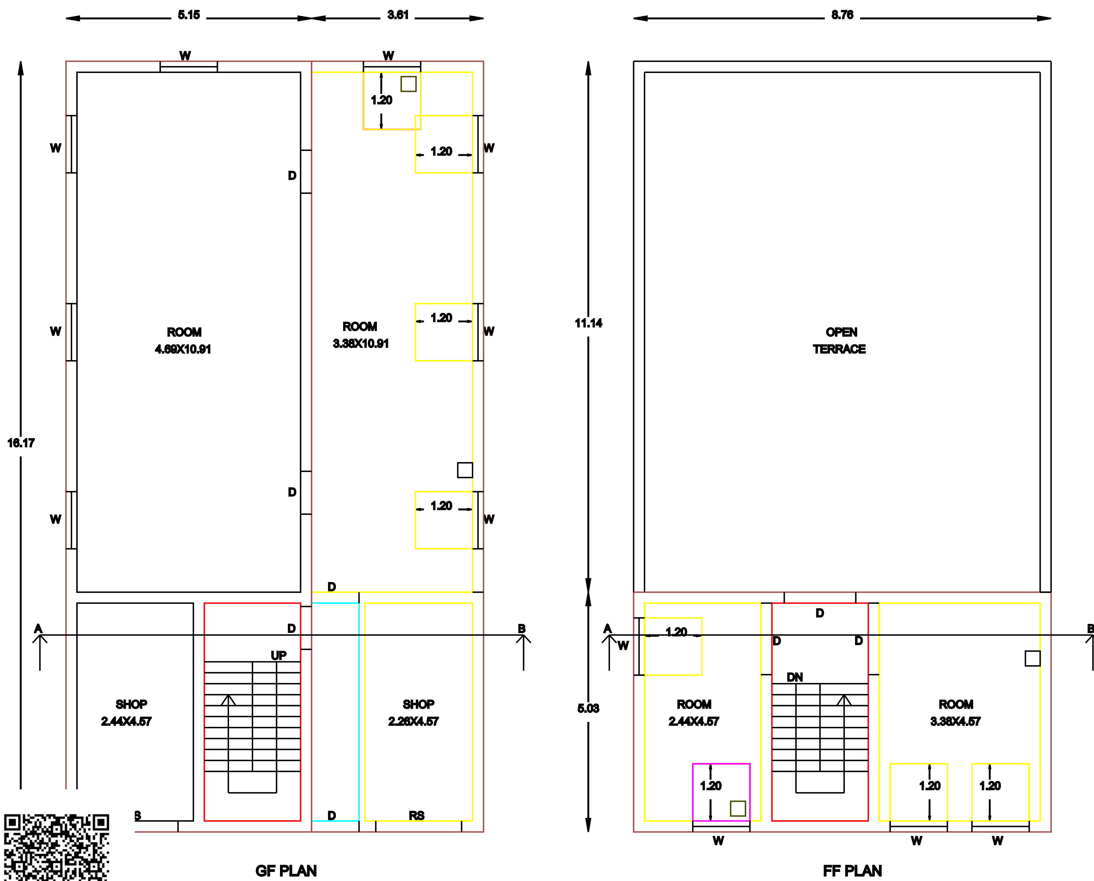
GF PLAN
