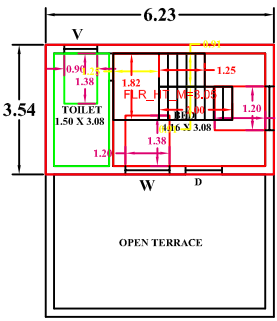
PRO. SECOND FLOOR PLAN
