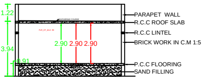
SECTION ON A-A
