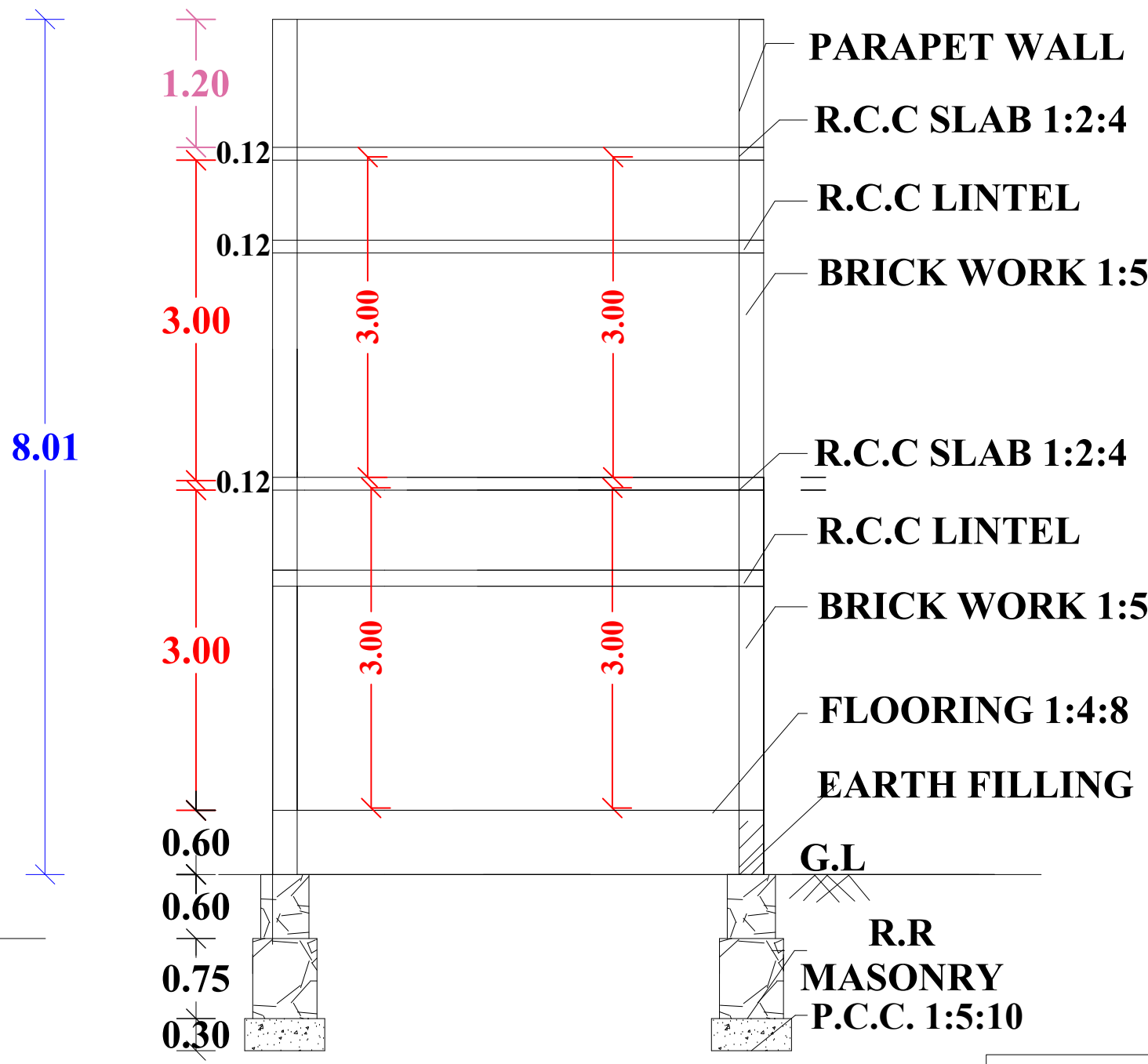
"SECTION "AB"
