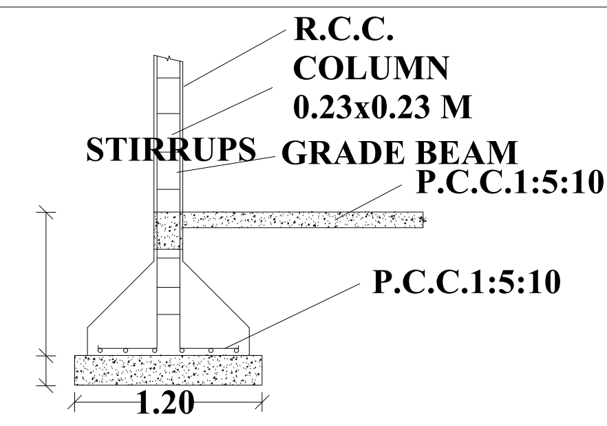
COLUMN DETAIL
