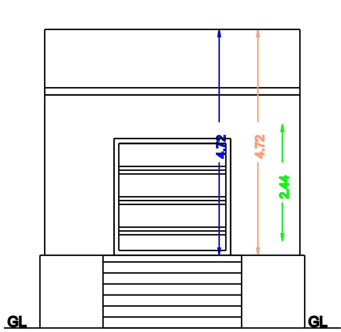
FRONT ELEVATION
