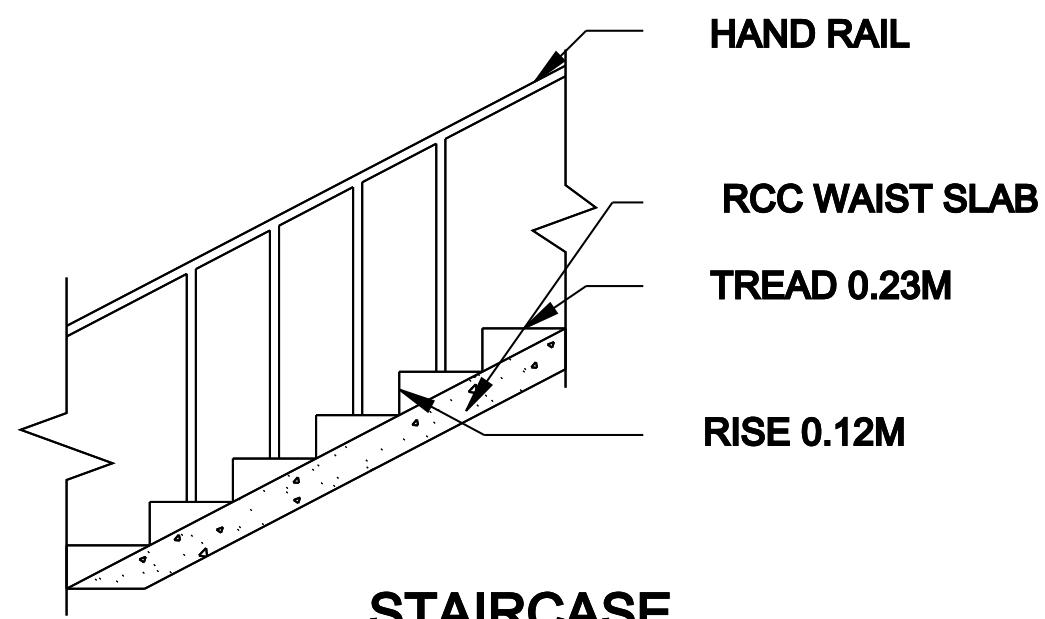
STAIRCASE
