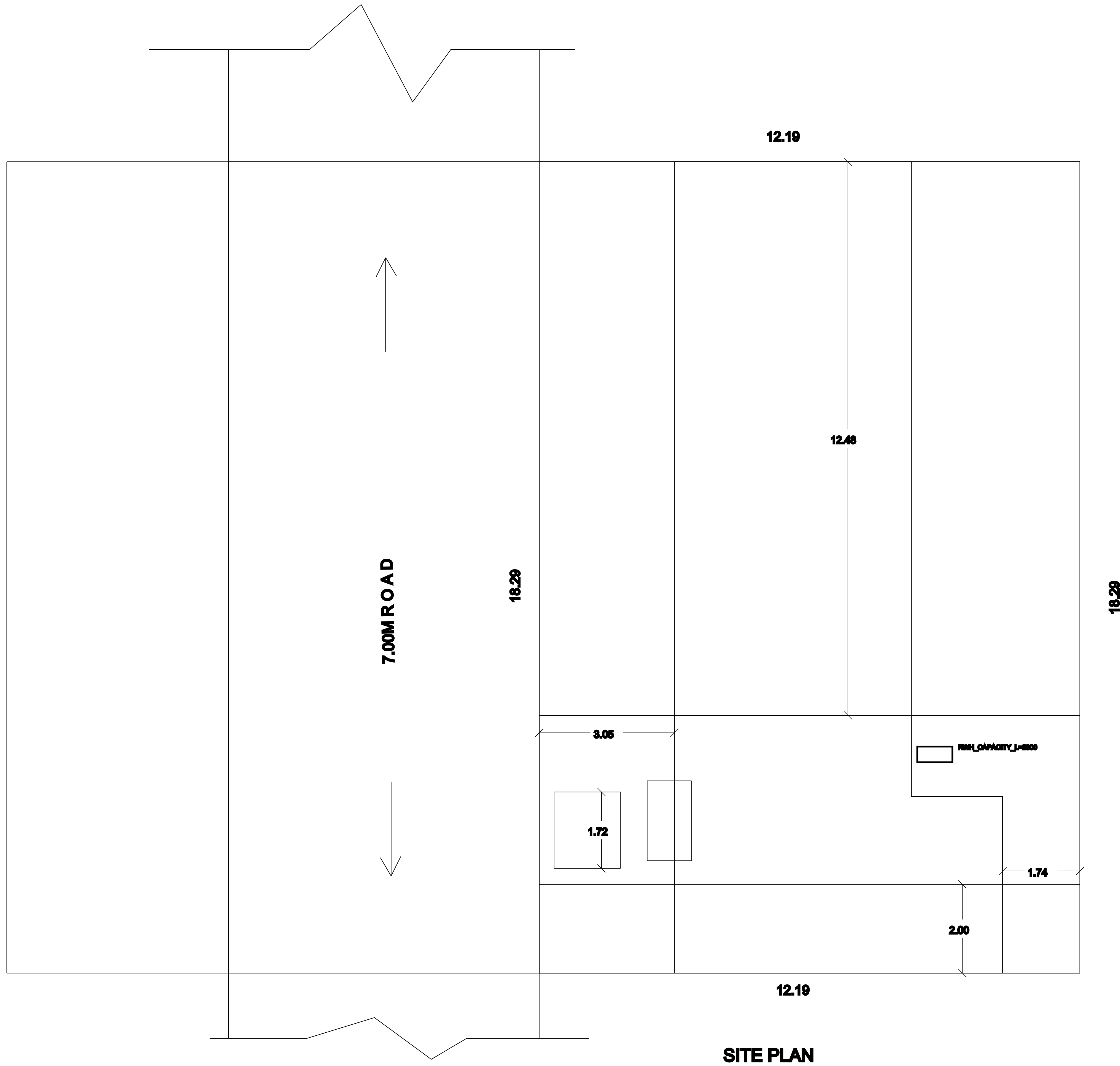
SITE PLAN
