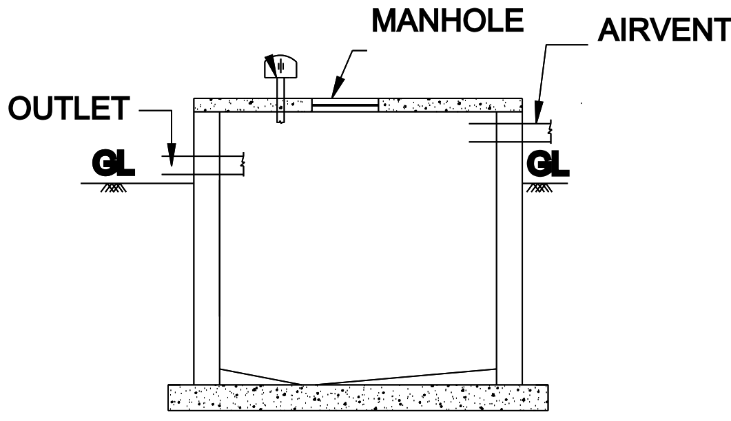
SECTION B-B'
