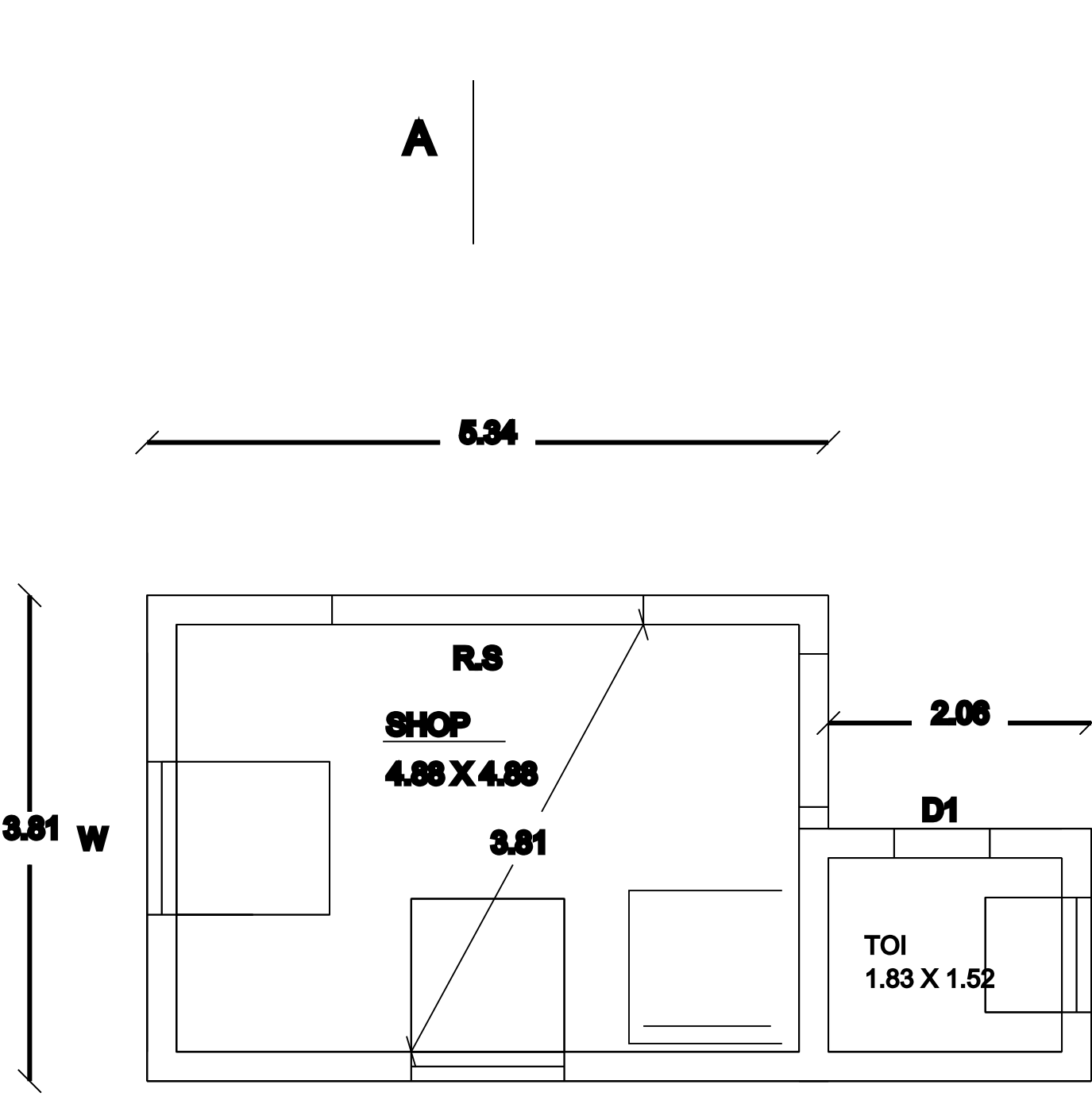
PLAN
