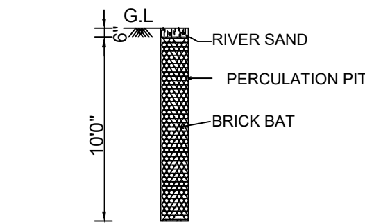
PERCULATION PIT
