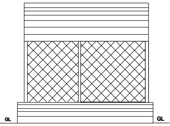
WEST FACE ELEVATION
