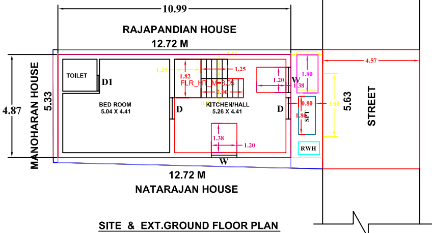
SITE & EXT.GROUND FLOOR PLAN
