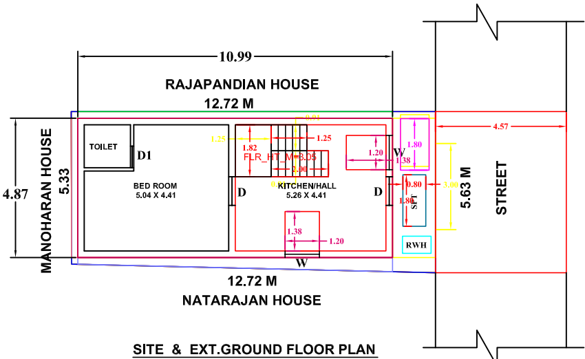
SITE & EXT.GROUND FLOOR PLAN
