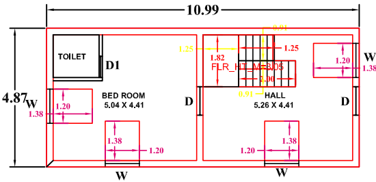
PLAN AT PRO. FIRST FLOOR
