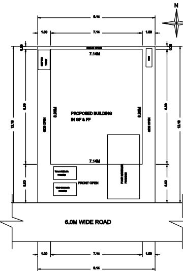
SITE PLAN
