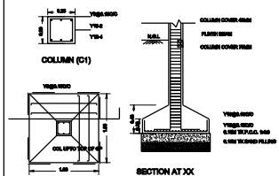
COLUMN DETAILS
