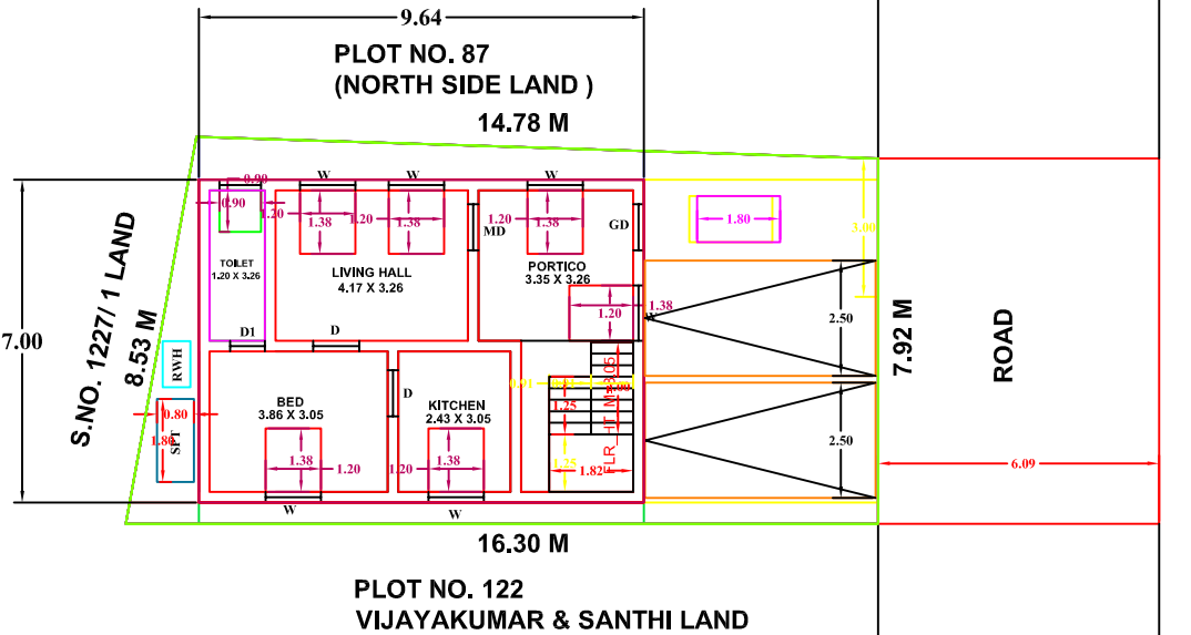
SITE & GROUND FLOOR PLAN
