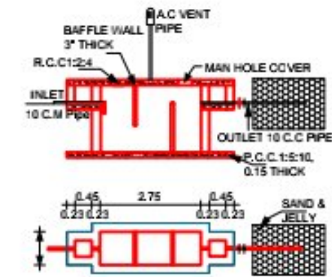
SEPTIC TANK AND TRECH
