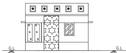
FRONT ELEVATION
