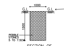
SCALE : 1" = 100
