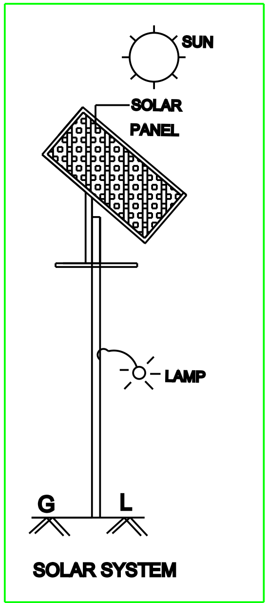
SOLAR SYSTEM
