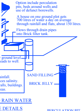
PERCOLATION PIT
