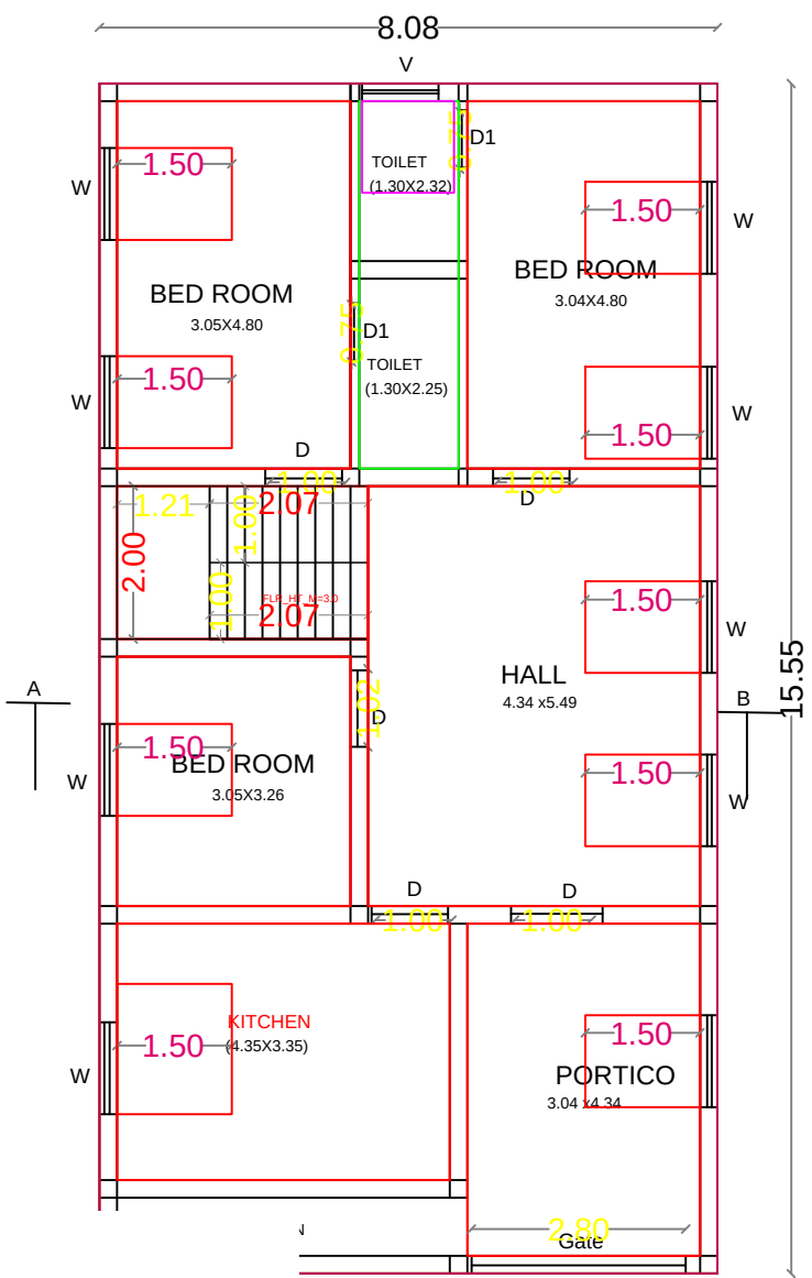
ID FLOOR PLAN
