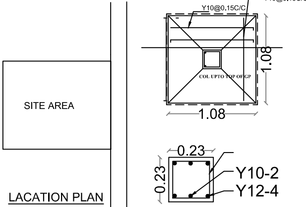
COLUMN (C1)
