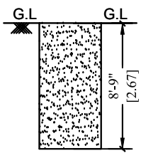
TRIAL PIT.
