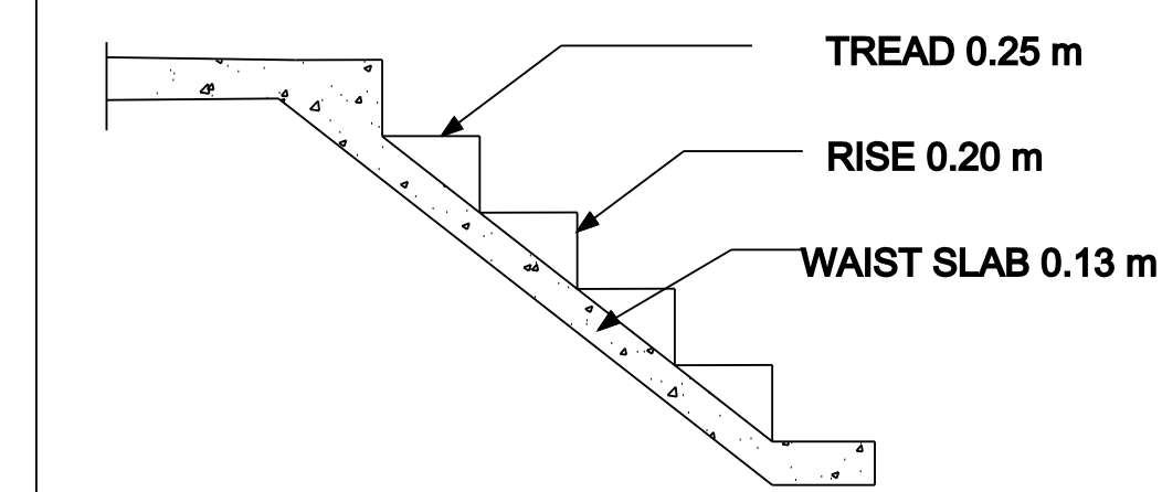
STAIR DETAILS
