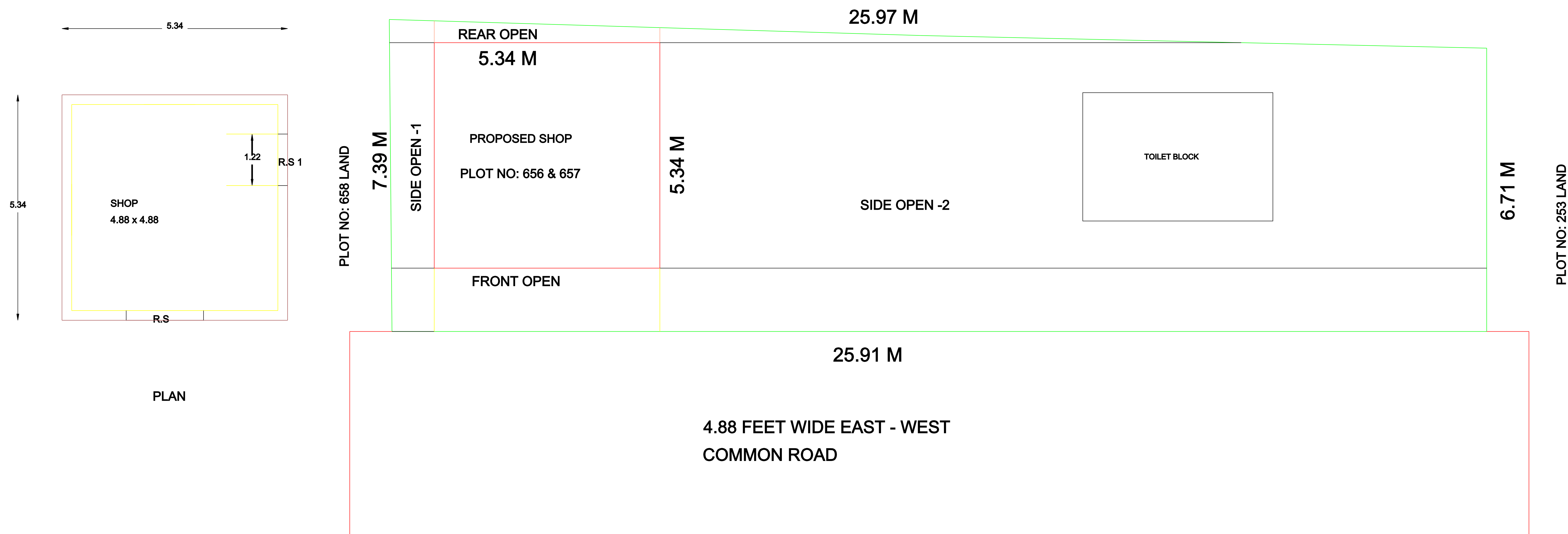
SITE PLAN
