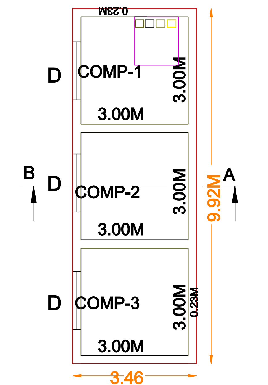
PLAN FOR SHED NO.54
