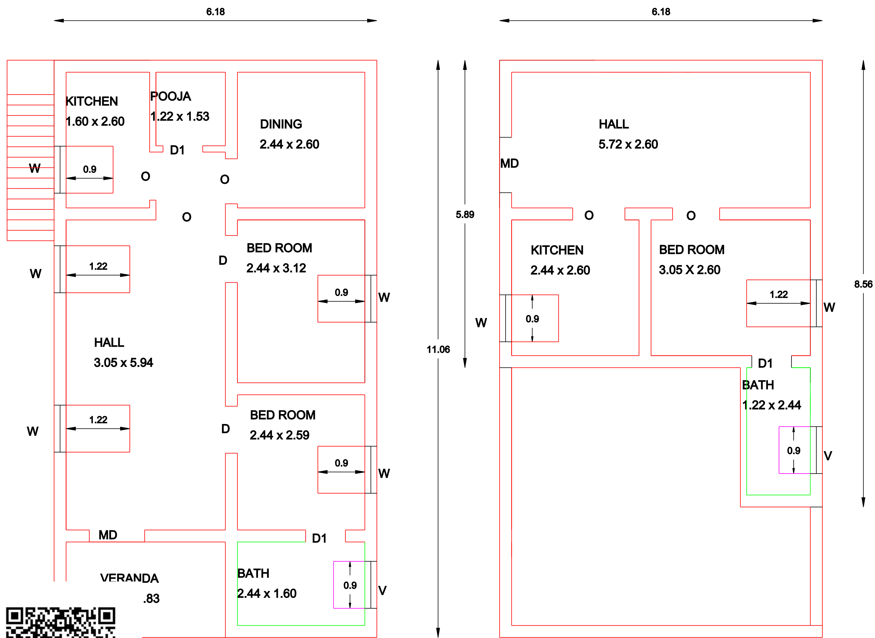
GROUND FLOOR
