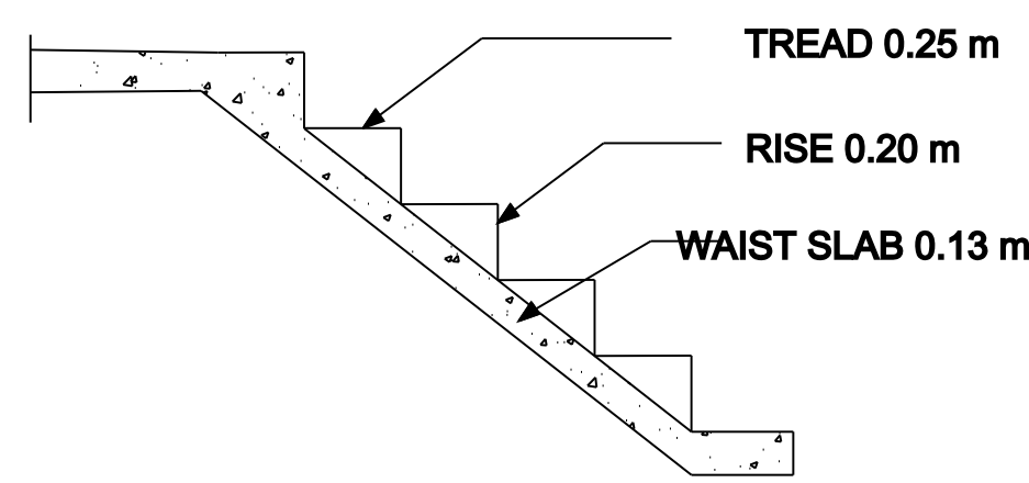
STAIR DETAILS
