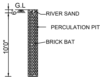
PERCOLATION PIT
