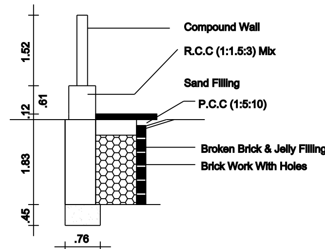
RAIN WATER HARVEST DETAILS
