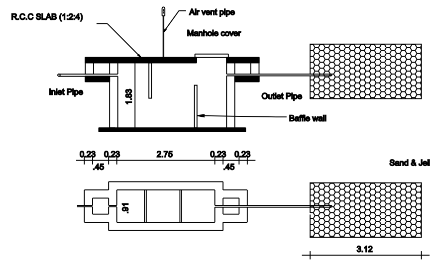
SEPTIC TANK & TRENCH
