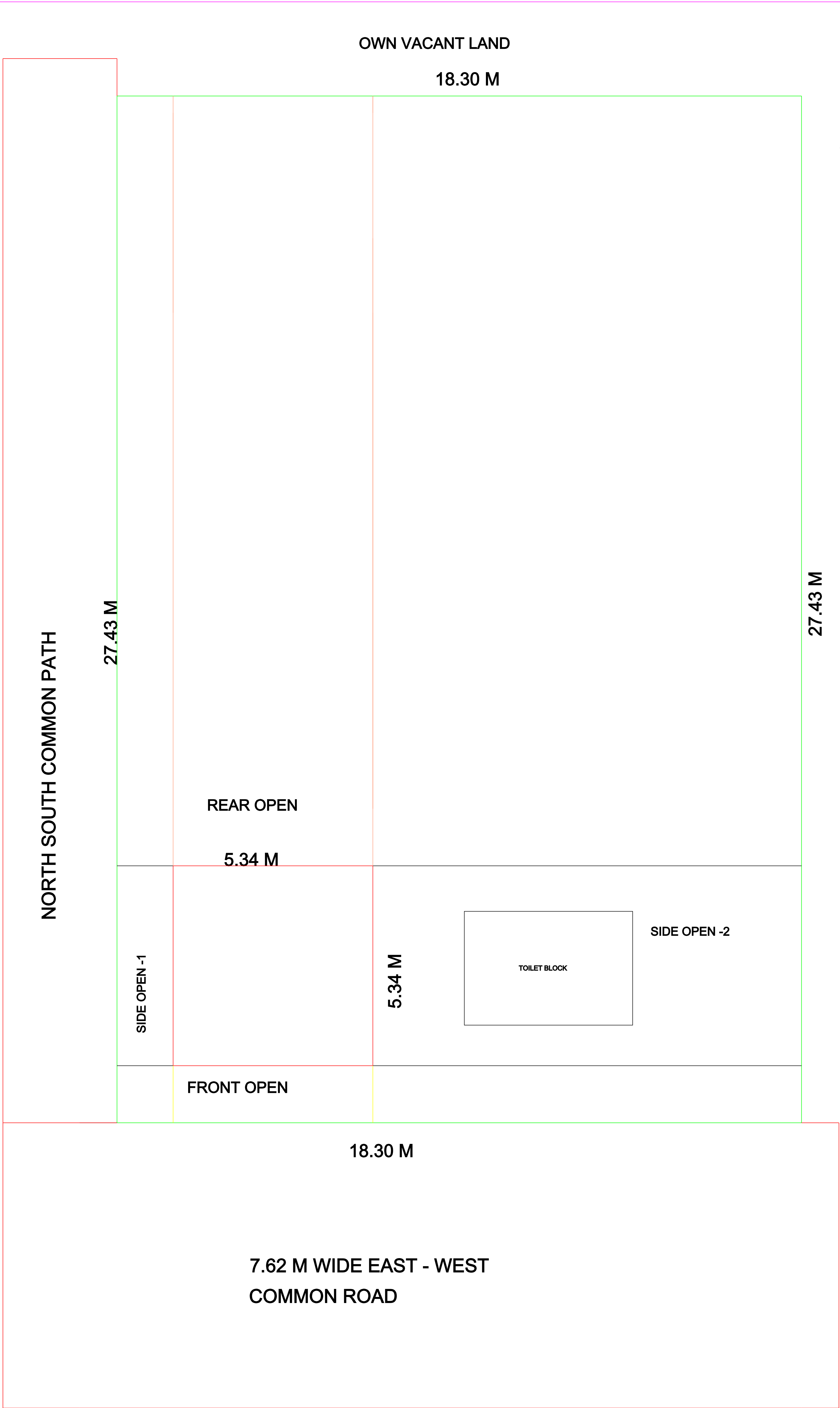
SITE PLAN
